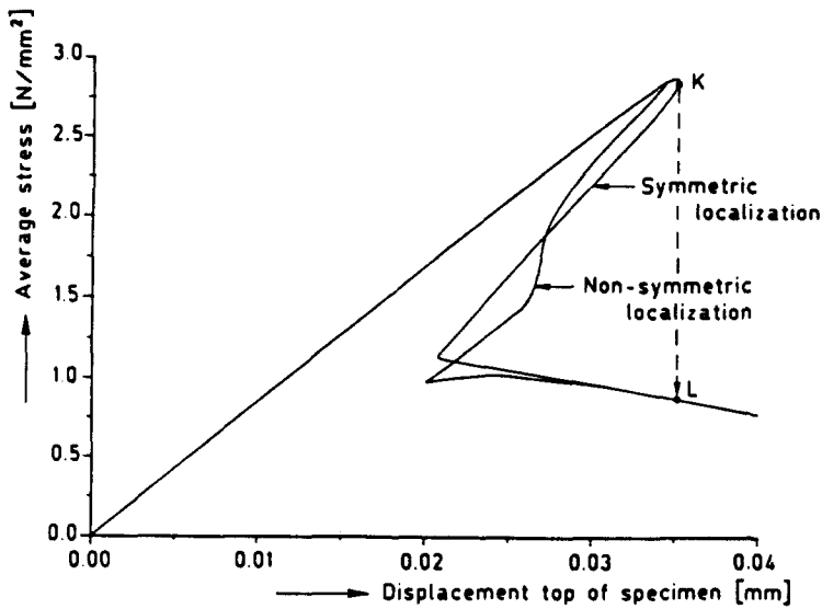
Fig. 10. Average stress as a function of the end displacement of the specimen.
