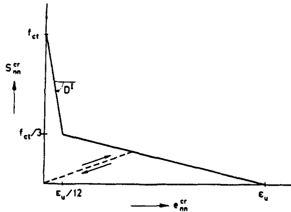
Fig. 2. Bilinear idealization of the normal stress in a crack as a function of the normal crack strain.
