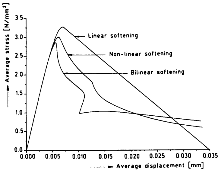
Fig. 8. Average stress as a function of the average deformations over a gauge length of 35 mm for different softening curves.
