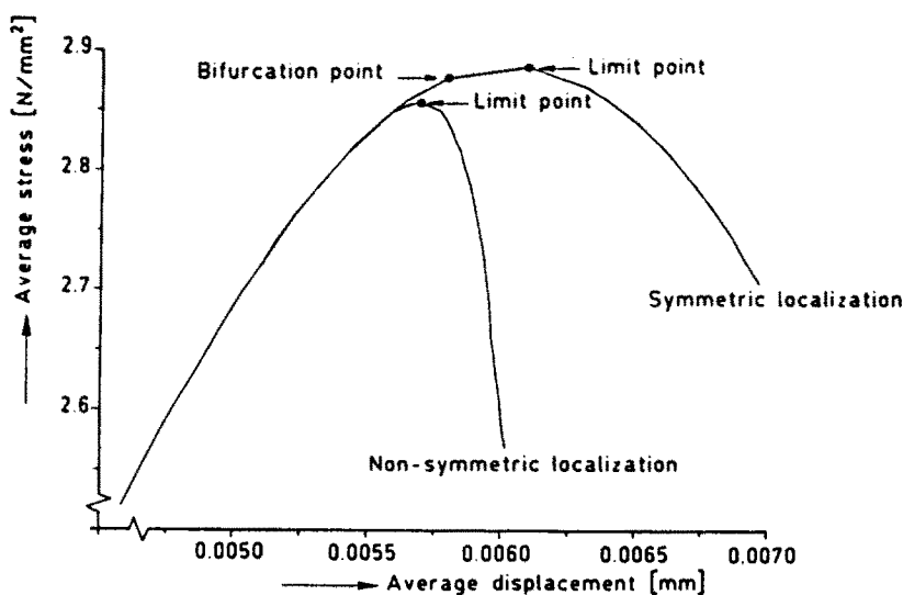
Fig. 6. Enlarged graph of the average stress as a function of the average deformations over a gauge length of 35 mm
