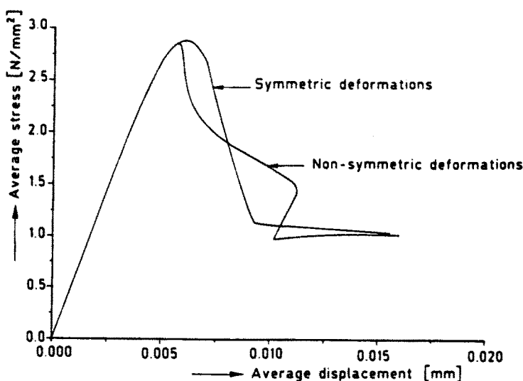
Fig. 5. Average stress as a function of the average deformations over a gauge length of 35 mm.
